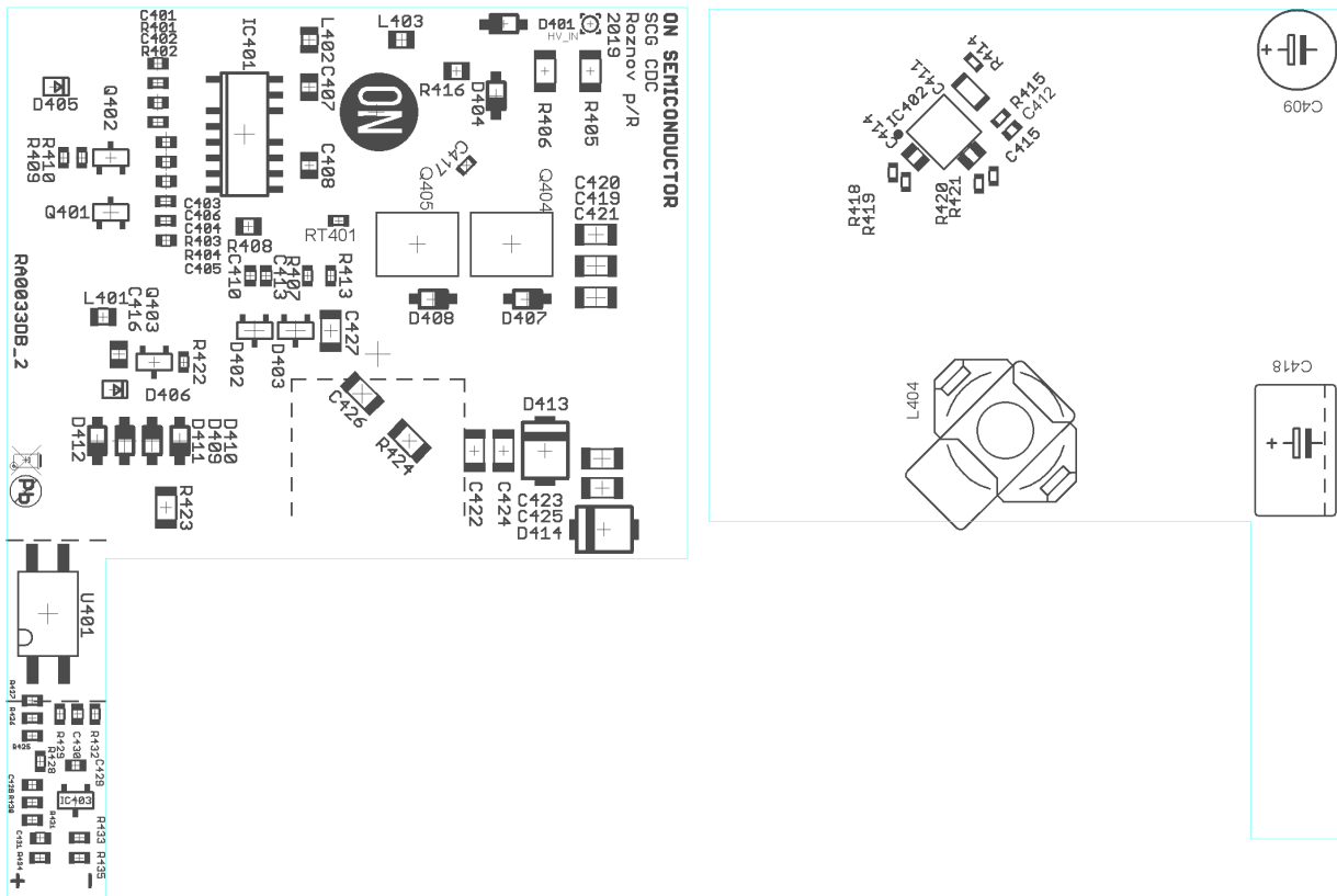
Figure 16. Top/ Bottom Layer PCB Layout and Assembly Plan of LLC STAGE MODULE MOD103
