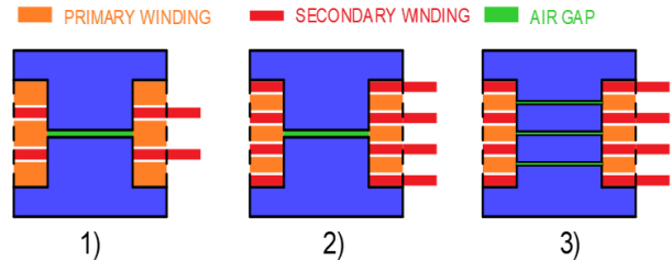
Figure 25. Hybrid Windings Transformer Possible Structures
