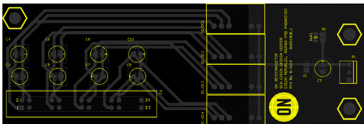
Figure 22. Top Overlay
