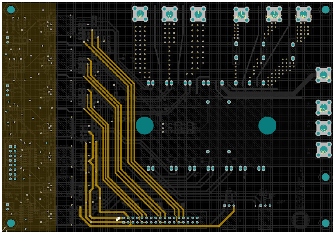
Figure 17. Signal Layer 1
