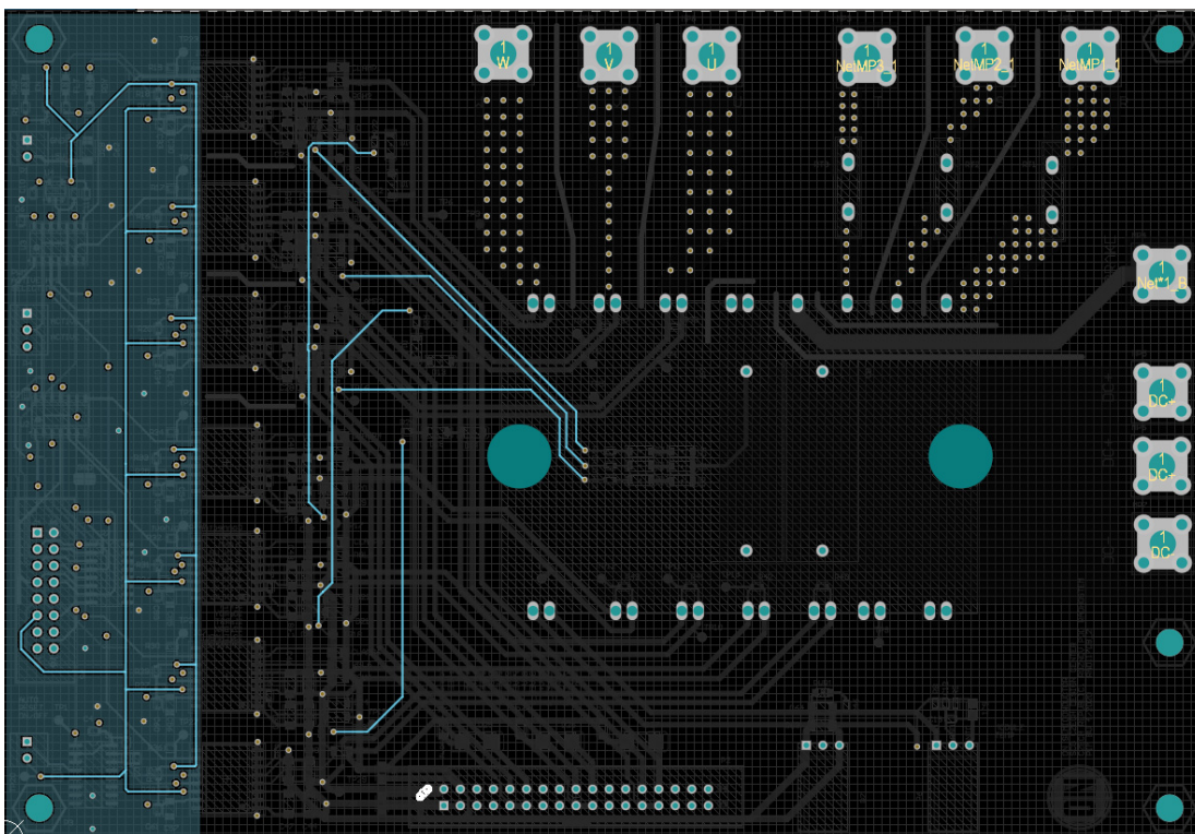
Figure 18. Signal Layer 2
