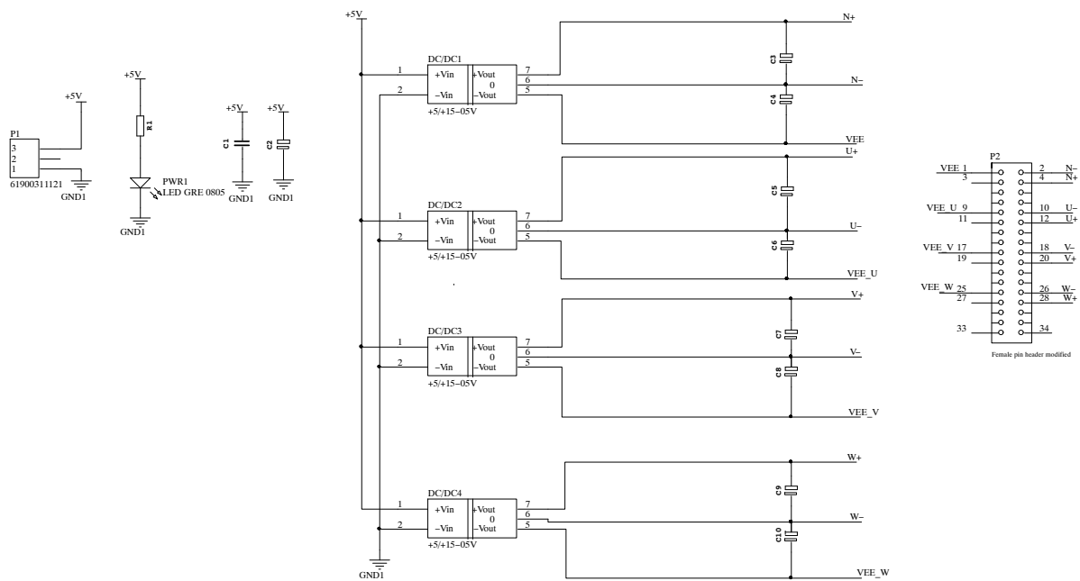
Figure 14. DC–DC Source Schematics
