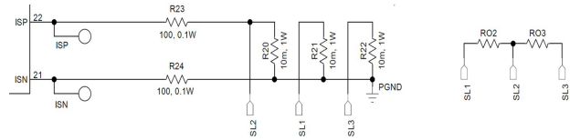
Figure 20. Shunt Resister Detection Schematic
