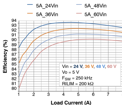
Figure 2. FAN65005A Efficiency
