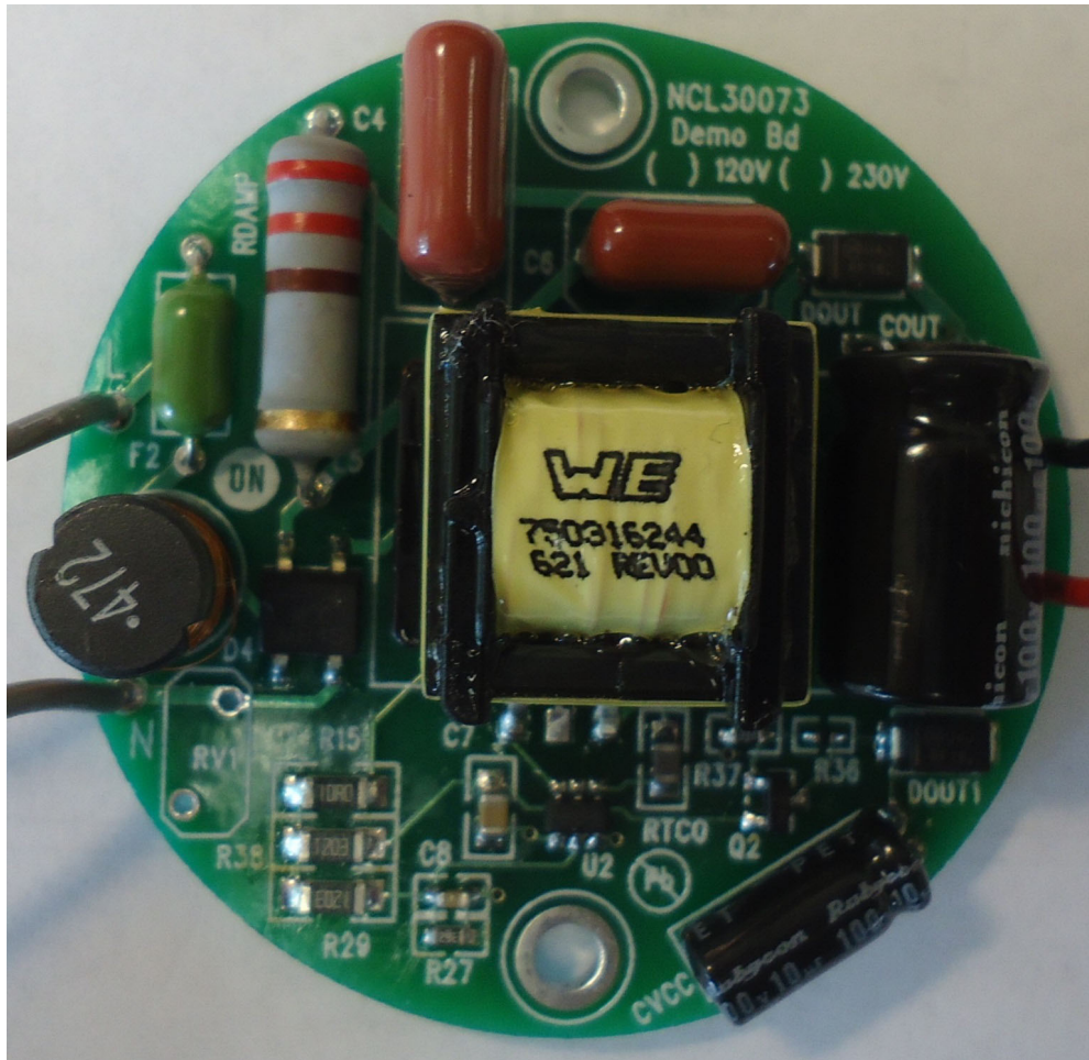
Figure 7. Top View
