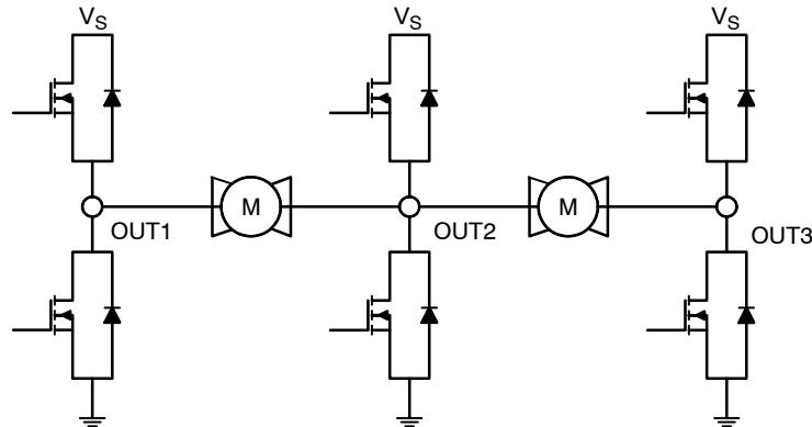
Figure 2. Cascaded Application
