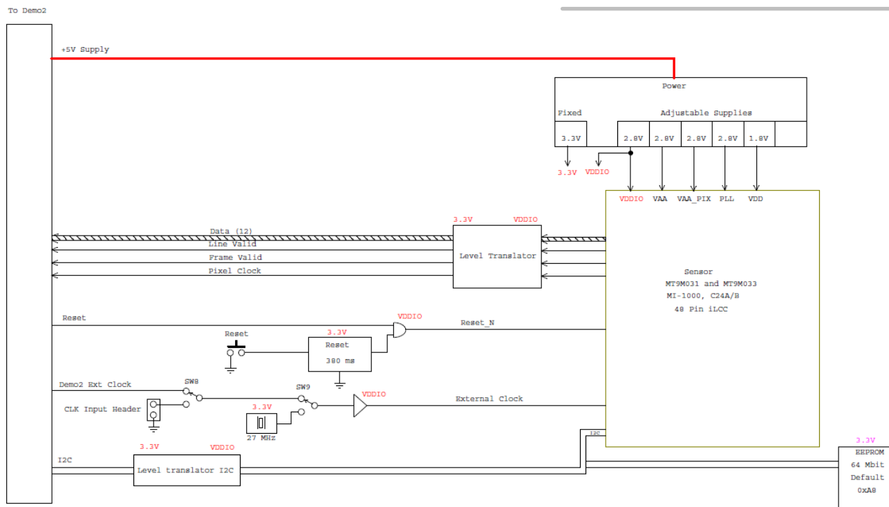
Figure 2. Block Diagram of MT9M031I12STCH-GEVB
