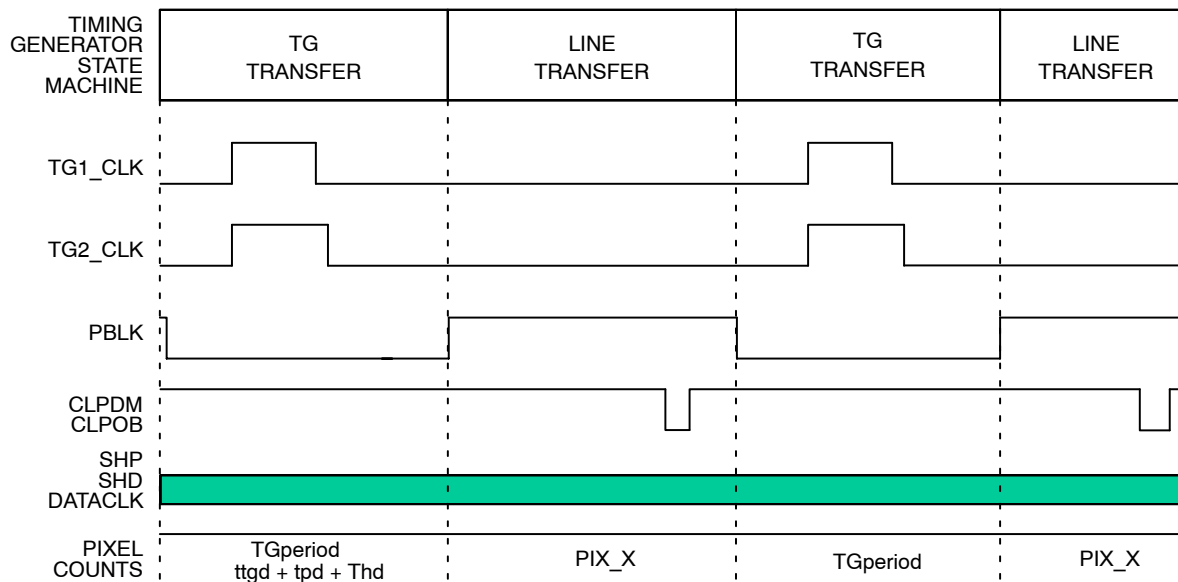
Figure 10. AD9845 Timing
