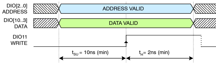
Figure 1. Programmable Register Timing
