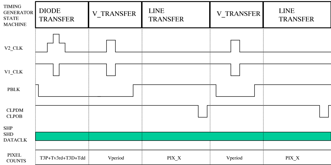
Figure 13. AD9845 Timing
