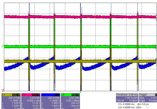
Figure 21. Skip Mode Operation Waveforms; C1 = V_{\text{Skip/latch}} , C2 = V_{\text{CC}} , C3 = V_{\text{FB}} , C4 = V_{\text{DRV}}
