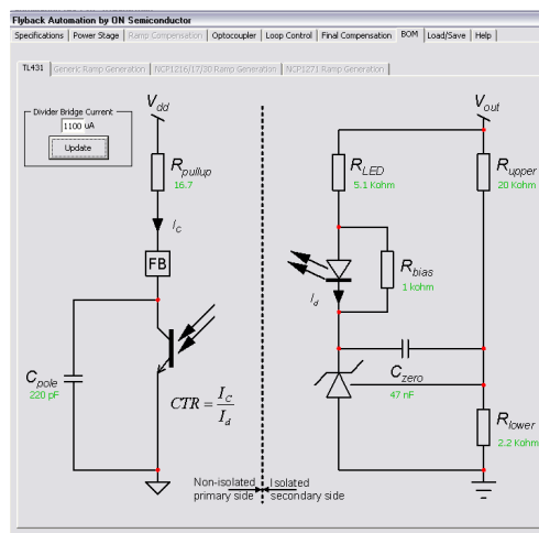
Figure 16. Screenshot of the Final Feedback Network Bill of Materials
