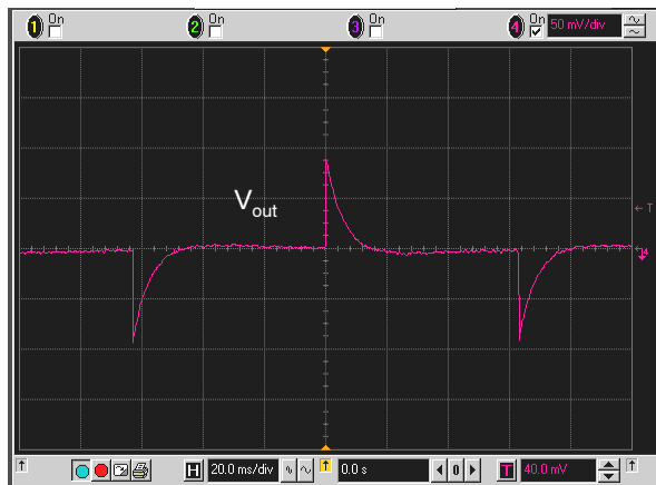
Figure 14. Load Step from 0.5 A to 3 A with a 1 A / \mu s Slew-rate from a 230 Vac source
