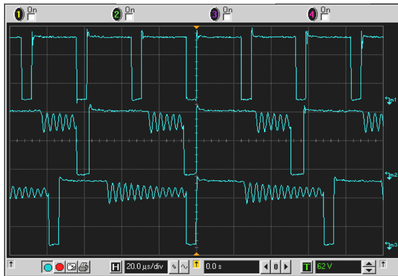
Figure 11. The Drain-source Waveform at Different Output Currents (3 A, 2 A and 1 A). The Input Voltage is 230 Vac
