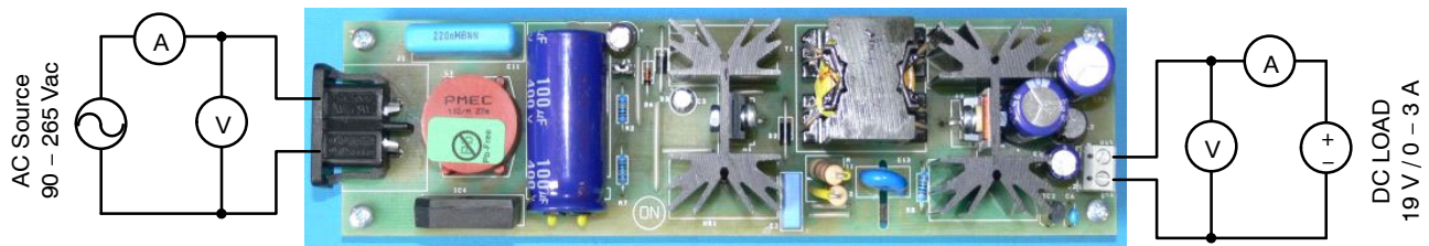
AC/DC 19 V – 3 A adapter
