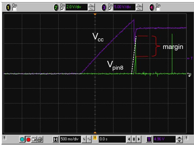
Figure 8. Startup Sequence to Test the Margin on the 100 ms Timer. V_{in} = 90 \text{ Vac} I_{out} = 3 \text{ A}
