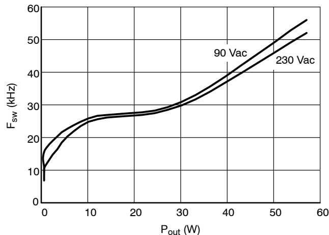
Figure 5. Switching Frequency F_{sw} vs. P_{out}
