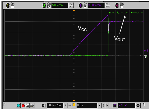
Figure 6. Startup time, V_{in} = 90 Vac
