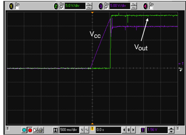
Figure 7. Startup time, V_{in} = 230 Vac
