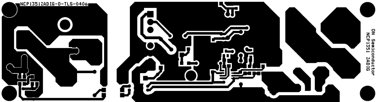
Figure 17. Copper Traces
