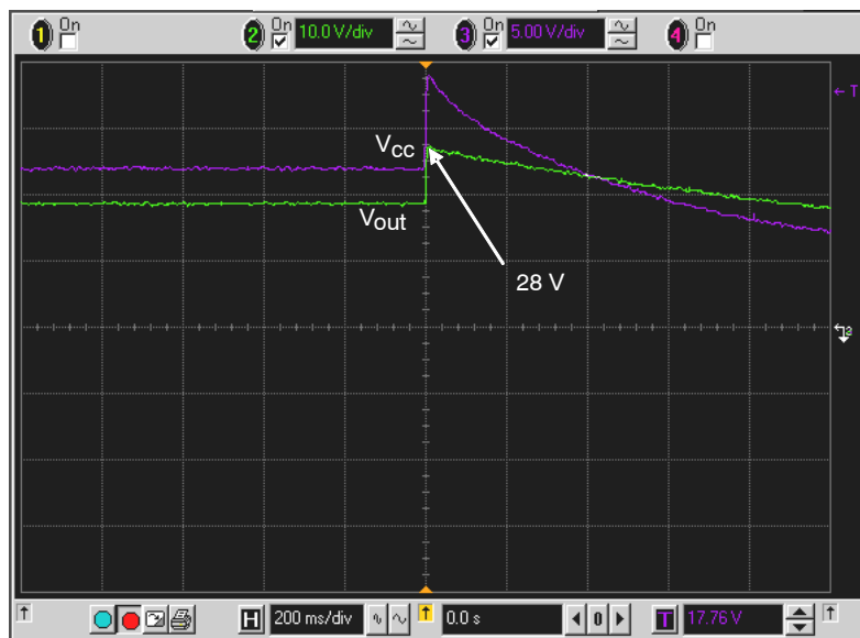
Figure 12. Short-circuit on the Optocoupler LED
