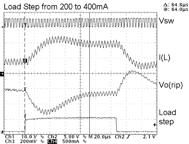
Figure 15. Transient Load
