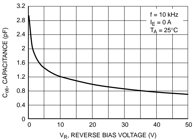
Figure 4. Output Capacitance
