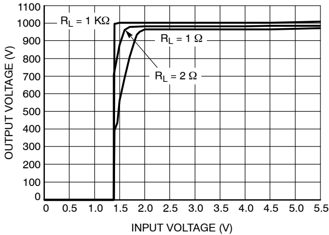
Figure 24. Dropout Characteristics
