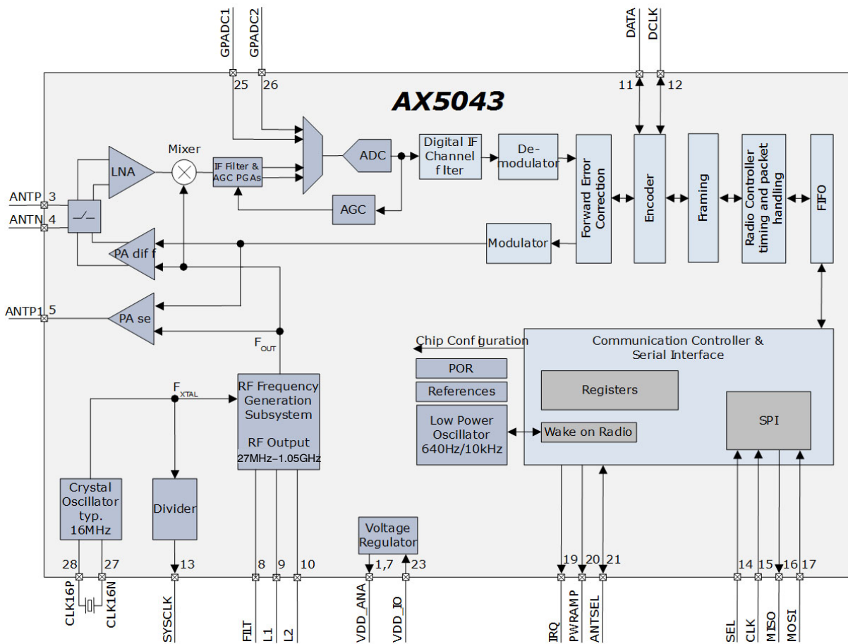
Figure 1. Block Diagram
