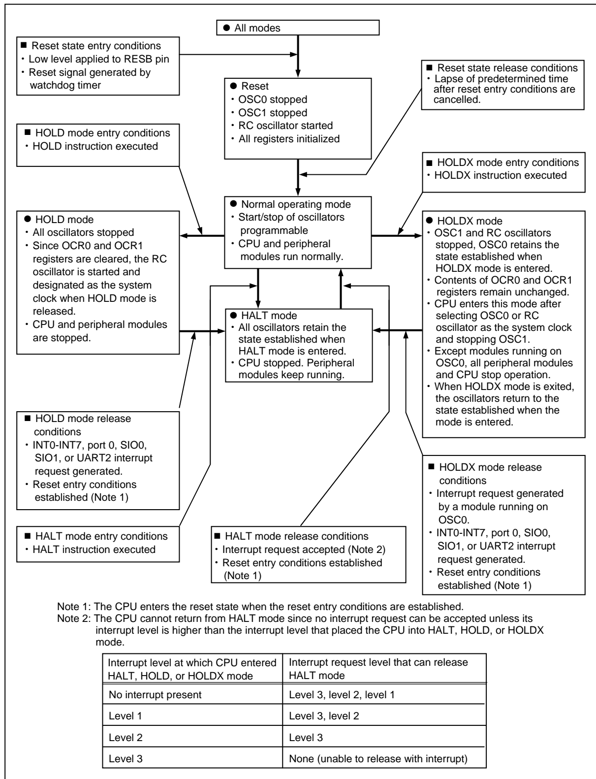
Figure 4.3.1 Standby Mode State Transition Diagram
