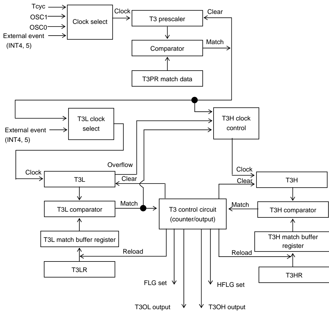
Figure 3.19.1 Timer 3 Block Diagram
