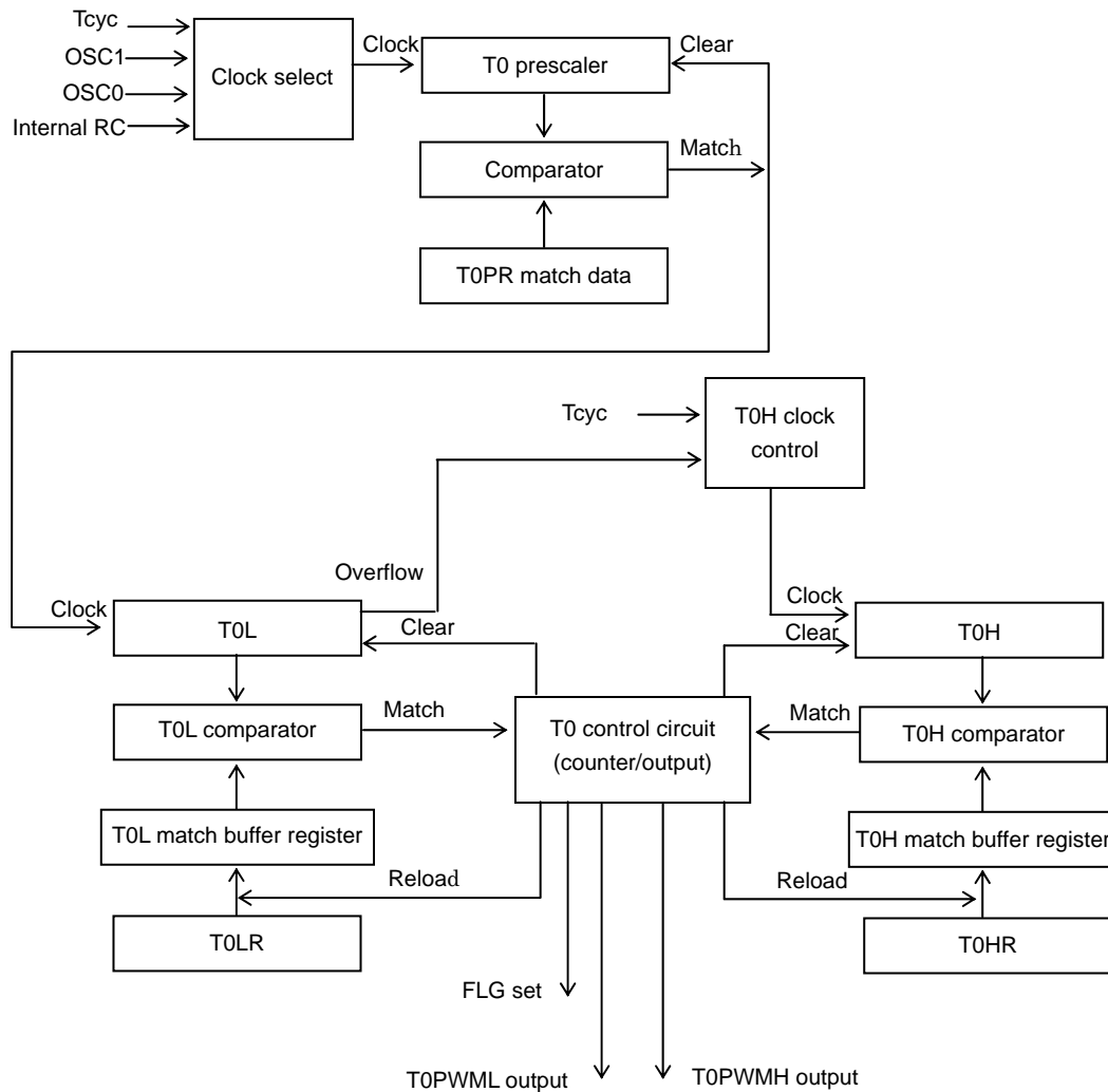
Figure 3.16.1 Timer 0 Block Diagram
