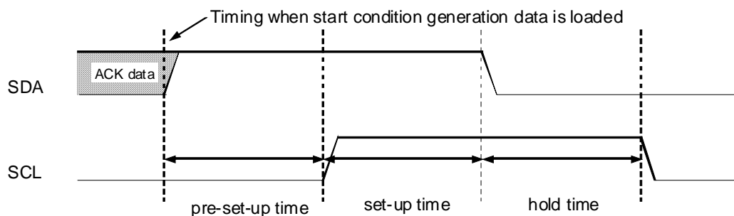
Figure 3.29.6 Restart Condition Generation Timing
