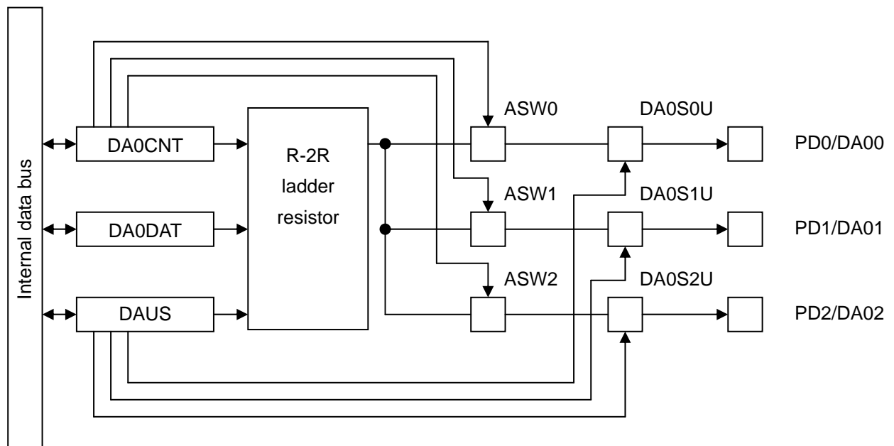
Figure 3.36.1 DA0 Block Diagram
