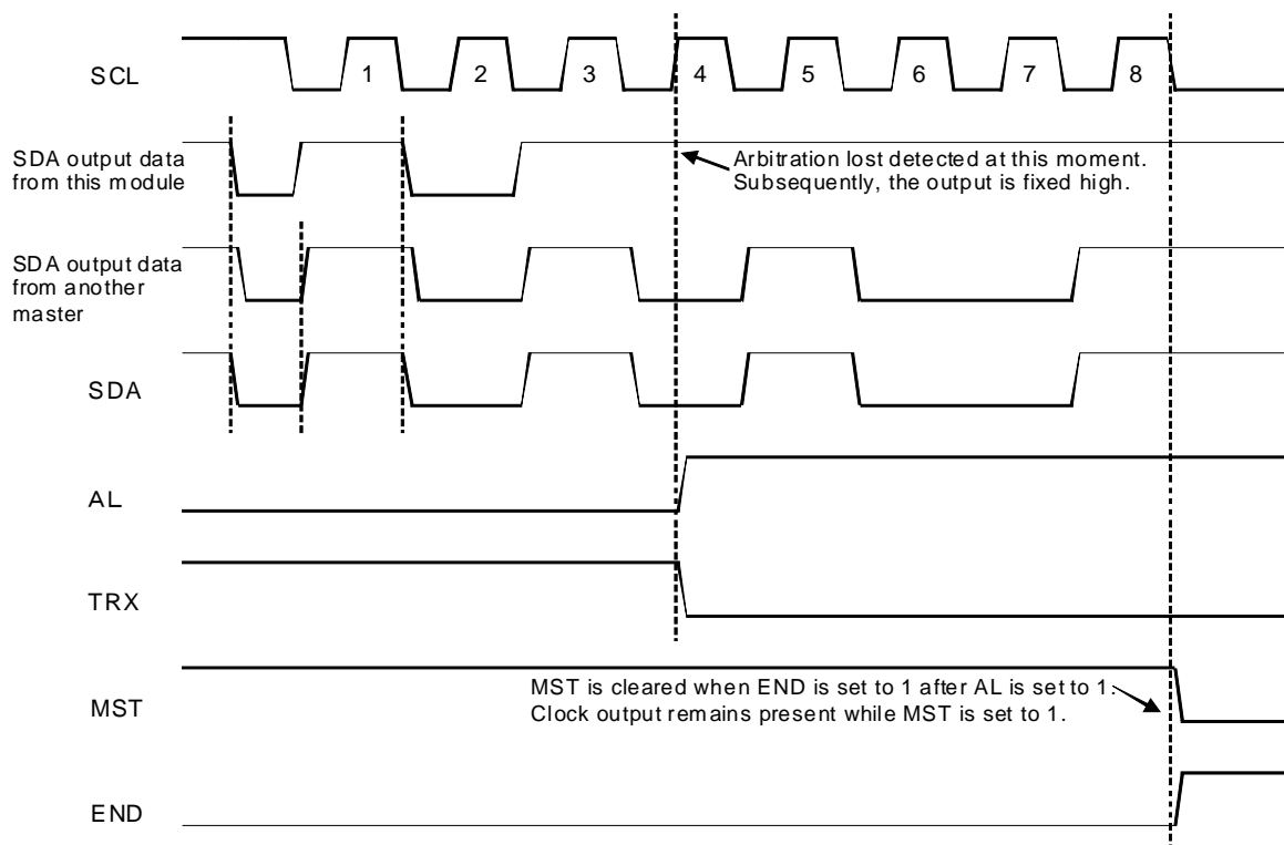
Figure 3.29.8 Arbitration Lost During Data Transfer
