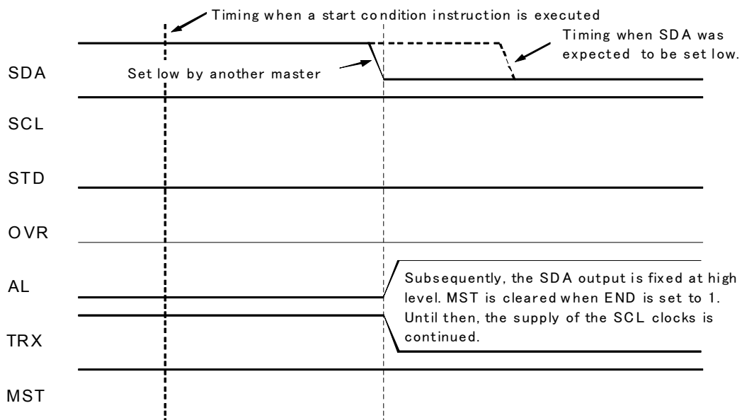
Figure 3.30.10 Arbitration Lost During Start Condition Generation <2>
