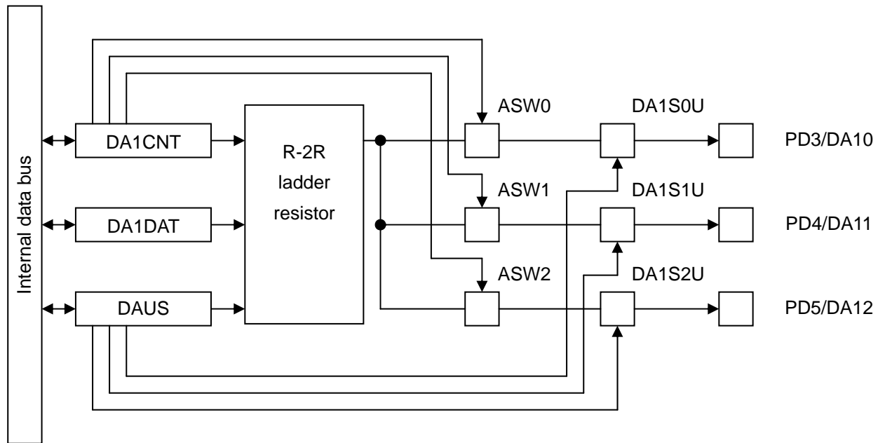
Figure 3.36.2 DA1 Block Diagram
