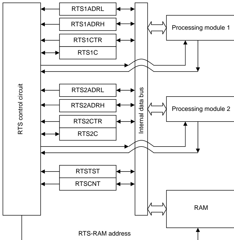
Figure 3.35.1 RTS Block Diagram
