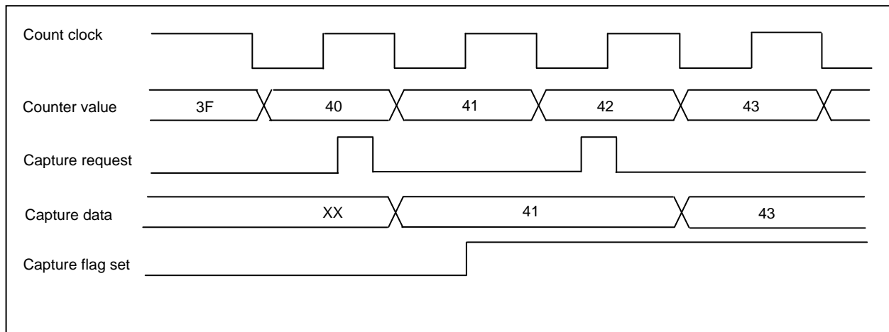
Figure 3.18.1 Capture Timing
