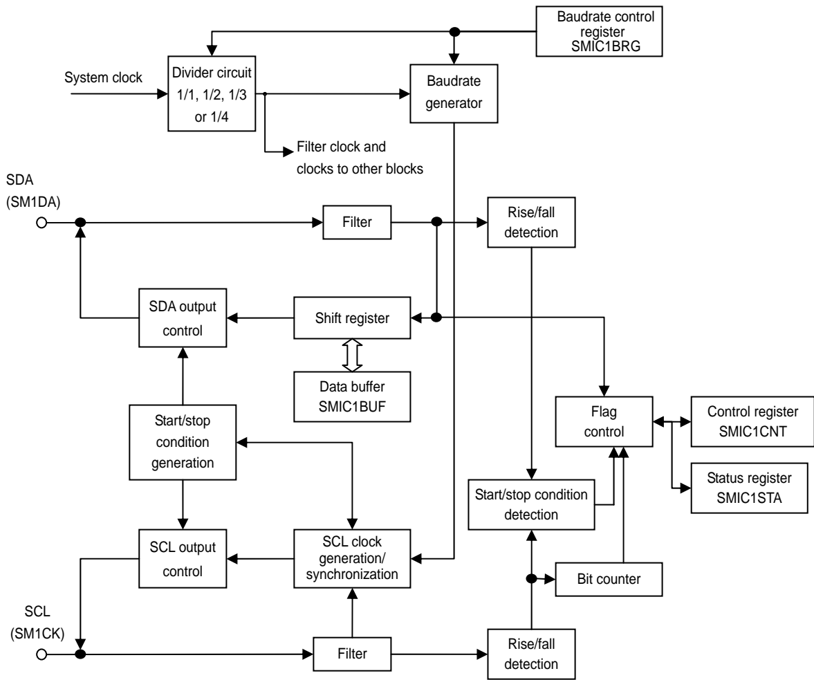
Figure 3.30.1 SMIIC1 Block Diagram
