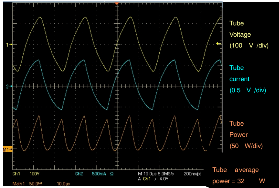
Figure 3. Tube Signals
