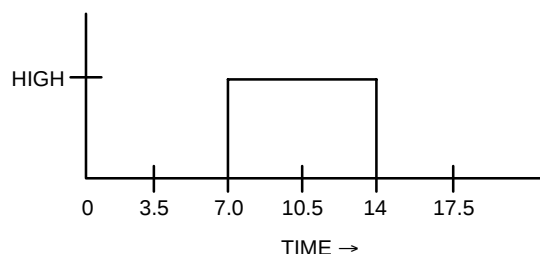
Figure 1. Output OE Pin for 1/2 Brightness
