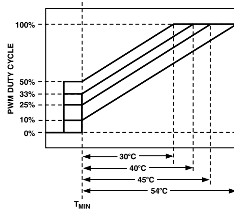
Figure 12. Increasing PWM_{MIN} Changes Effective T_{RANGE}
