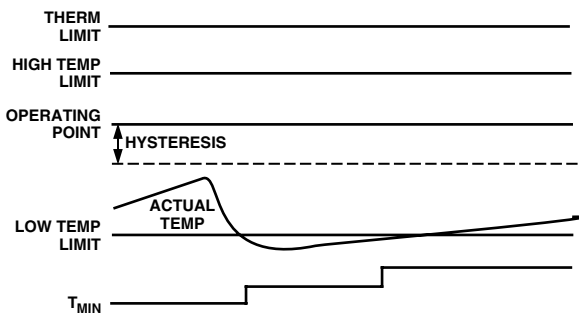
Figure 27. Increasing T_{MIN} for Quieter Operation
