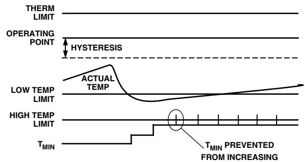
Figure 28. T_{MIN} Adjustments Limited by the High Temperature Limit
