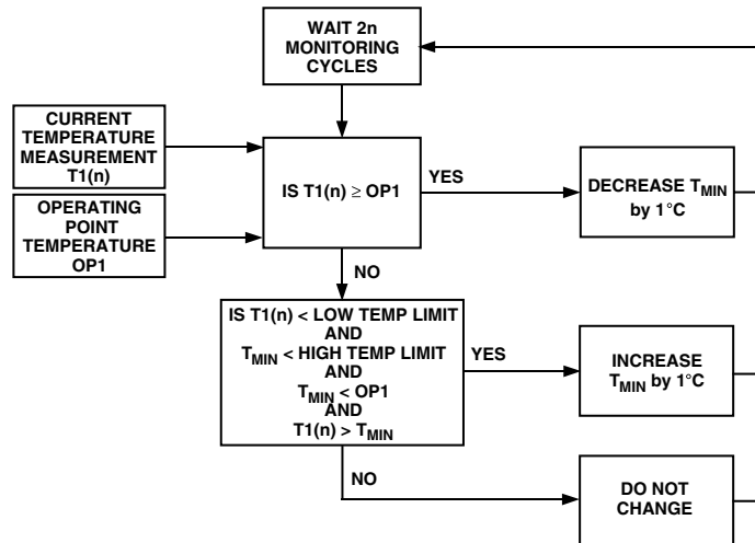
Figure 24. Long Cycle
