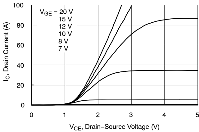
Figure 1. Typical Output Characteristics ( 25^\circ\text{C} )
