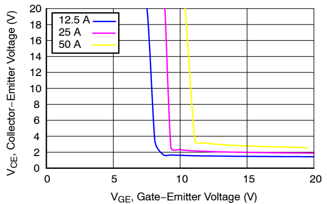
Figure 6. Saturation Voltage vs. V_{GE} ( 175^\circ\text{C} )
