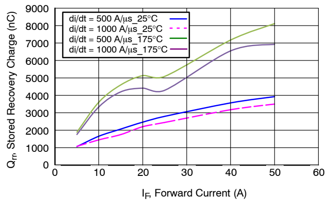
Figure 18. Stored Charge
