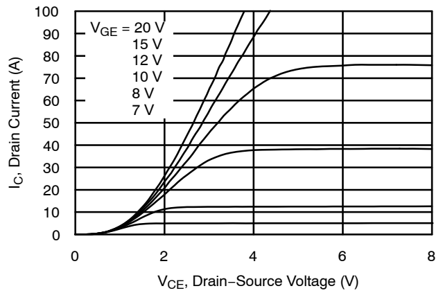
Figure 2. Typical Output Characteristics ( 175^\circ\text{C} )
