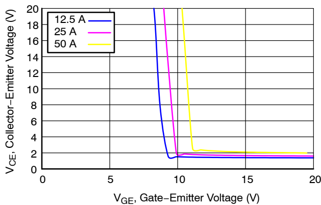
Figure 5. Saturation Voltage vs. V_{GE} ( 25^\circ\text{C} )
