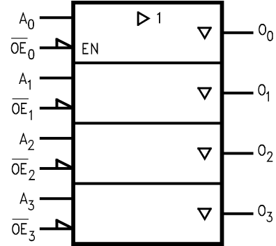
Figure 2. Logic Symbol
