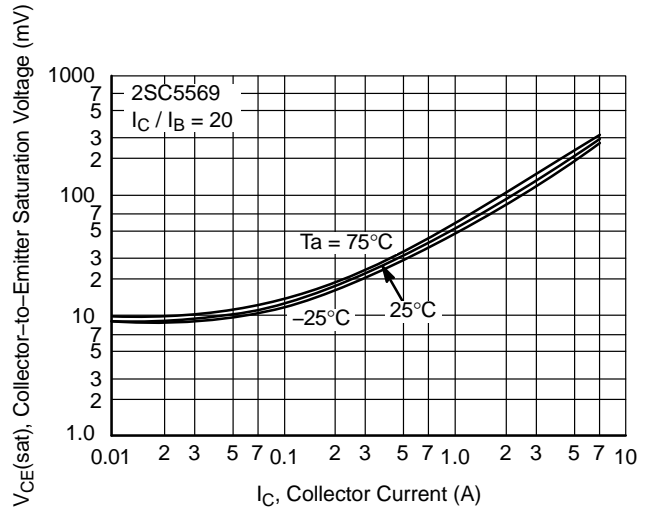
Figure 9. V_{CE(sat)} - I_C
