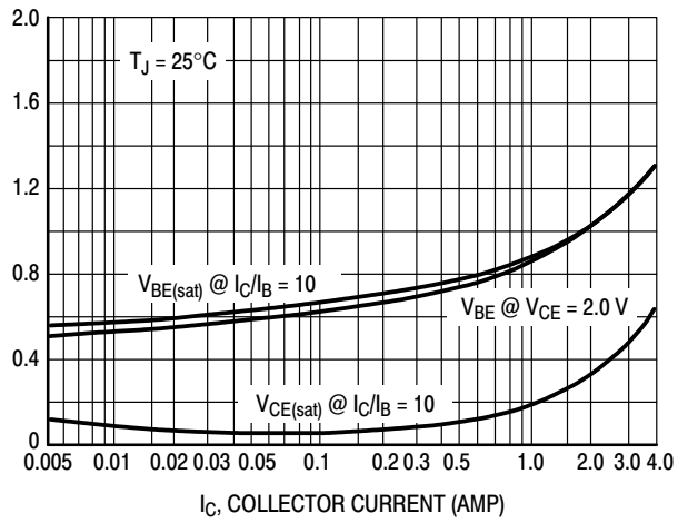
Figure 3. "On" Voltages
