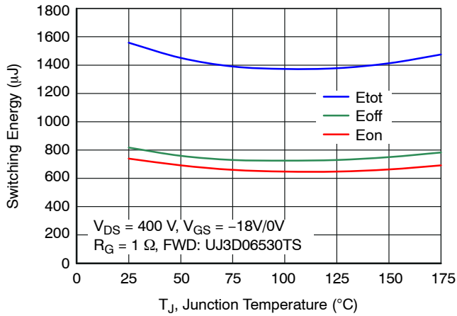
Figure 19. Clamped Inductive Switching Energy vs. Junction Temperature at I_D = 60\text{ A}
