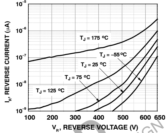
Figure 3. Reverse Characteristics
