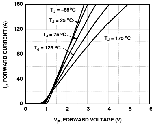
Figure 2. Forward Characteristics
