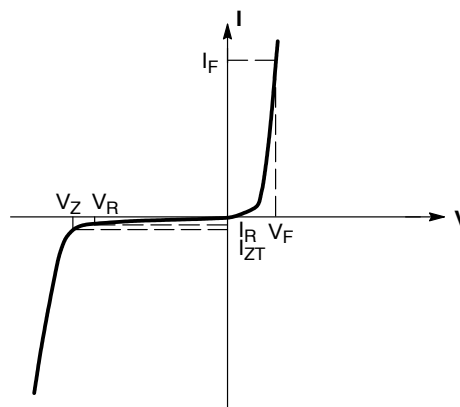
Figure 1. Uni-directional Zener
