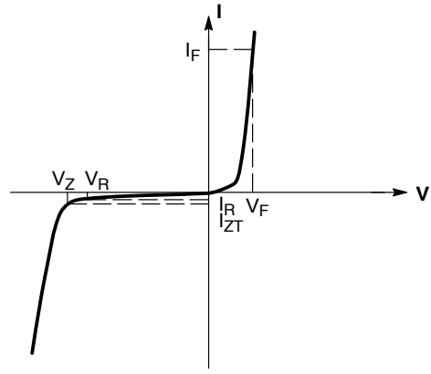
Figure 1. Uni-directional Zener
