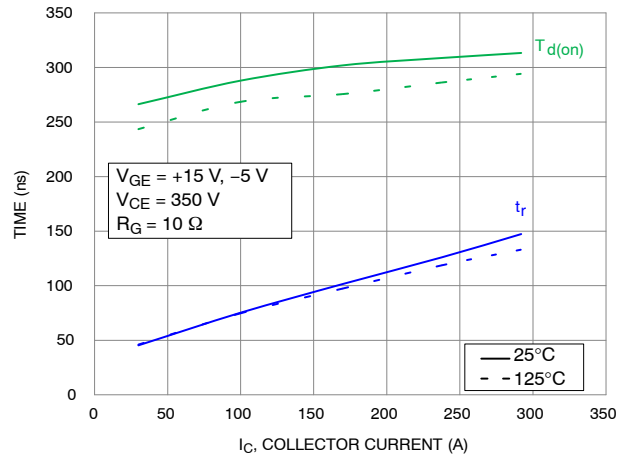
Figure 9. Typical Turn-On Switching Time vs. I_C
