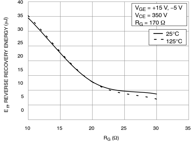
Figure 15. Typical Reverse Recovery Energy Loss vs. R_G
