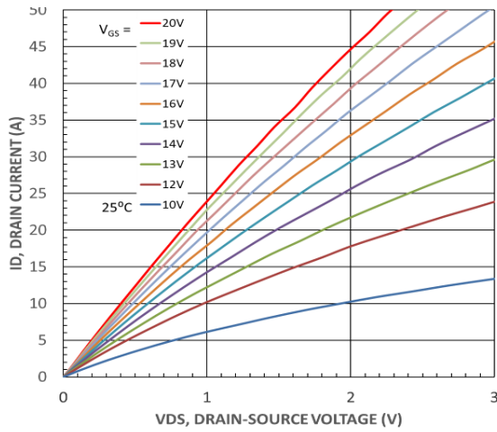
Figure 2. MOSFET Typical Output Characteristics
