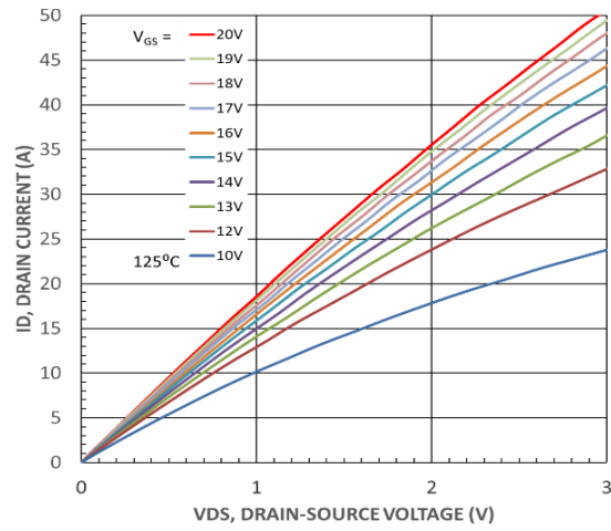
Figure 3. MOSFET Typical Output Characteristics
