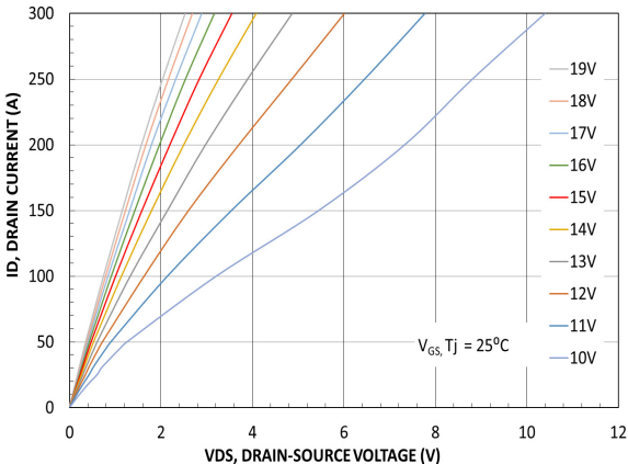
Figure 2. MOSFET Typical Output Characteristics
