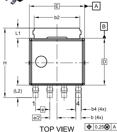
TOP VIEW \text{M} \begin{matrix} \text{A} \\ 0.25 \end{matrix}
