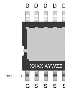
TCPAK57 CASE 760AG
