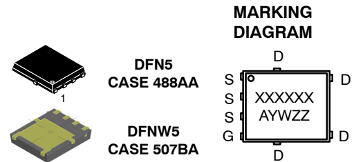
N-CHANNEL MOSFET
