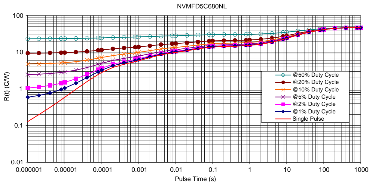
Figure 13. Thermal Characteristics
