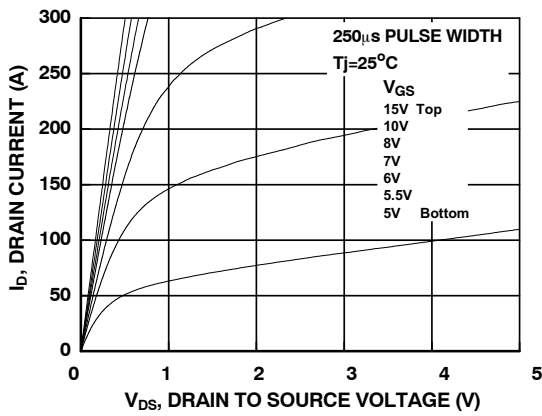
Figure 9. Saturation Characteristics
