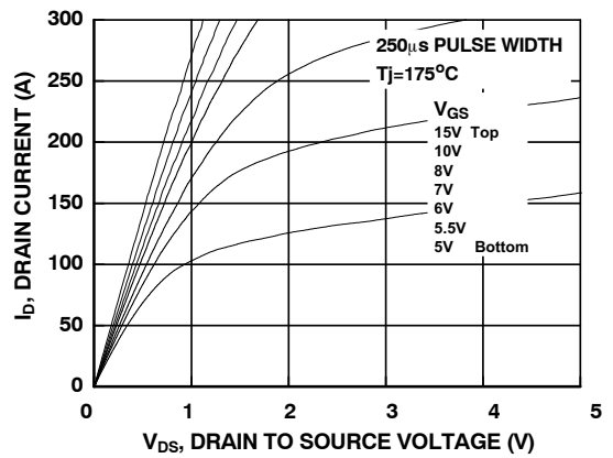
Figure 10. Saturation Characteristics
