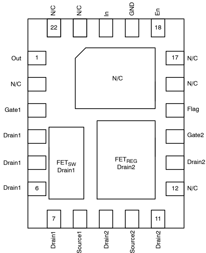
(Top View)
