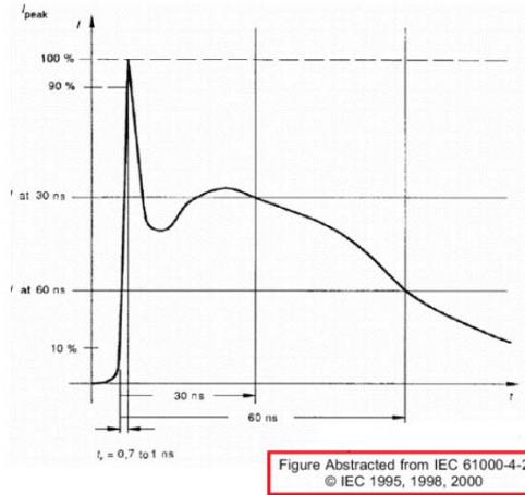
Figure 29. IEC 61000-4-2 Curve
