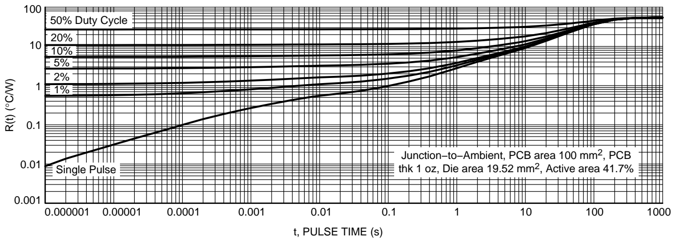
Figure 9. Thermal Characteristics
