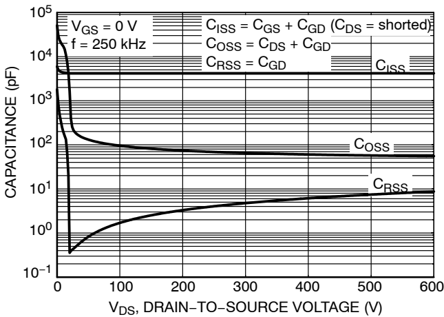
Figure 5. Capacitance Characteristics
