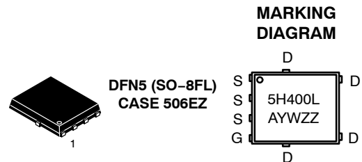
N-CHANNEL MOSFET
