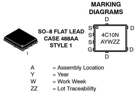
N-CHANNEL MOSFET
