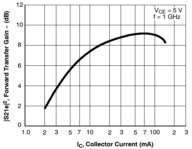
Figure 6. |S_{21e}|^2 - I_C
