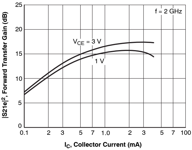
Figure 5. |S_{21e}|^2 - I_C
