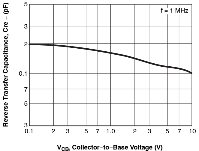
Figure 4. C_{re} - V_{CB}
