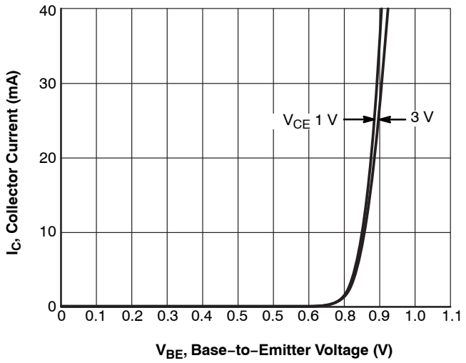
Figure 2. I_C - V_{BE}
