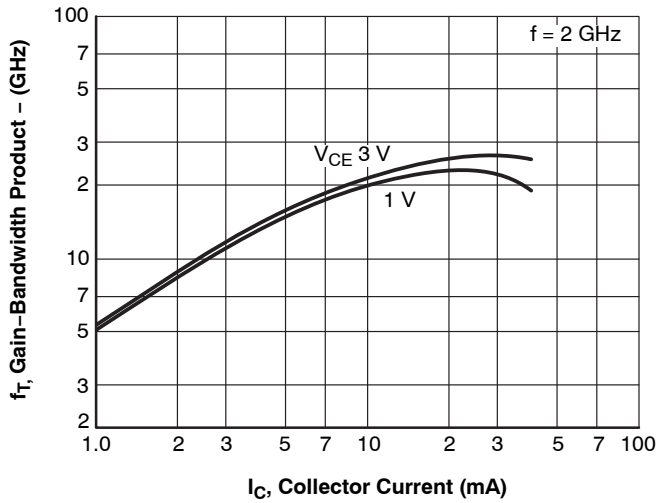
Figure 6. f_T - I_C
