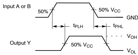
Figure 4. Switching Waveforms
