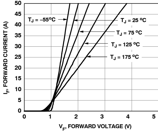
Figure 1. Forward Characteristics
