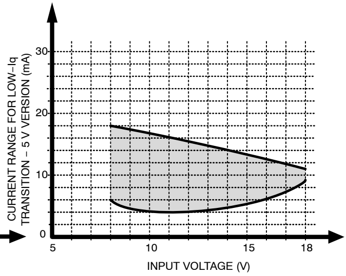
Figure 26. Switcher to Low-Iq Mode Transition (5.0 V Version, 2.2 \mu H) vs. Input Voltage
