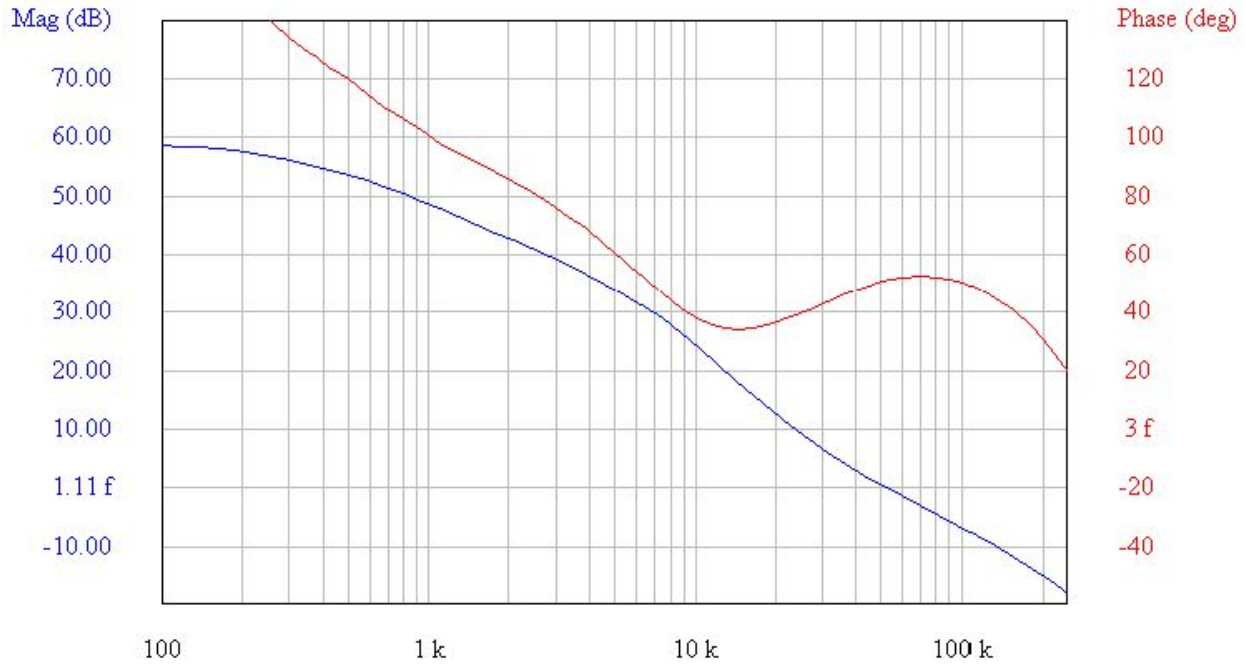
Figure 30. Bode Plot of the Open Loop Transfer Function of a Buck Converter using the NCV891330 for V_{in} = 13\text{ V} , V_{out} = 3.3\text{ V} , I_{out} = 2\text{ A} , C_{out}=3 \times 10\ \mu\text{F} and L=2.2\ \mu\text{H}
