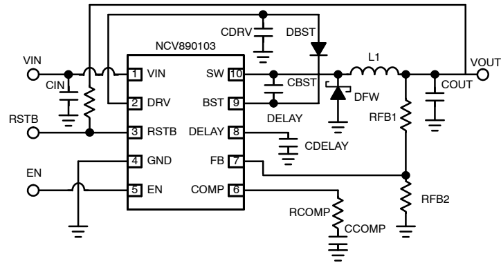
Figure 1. Typical Application
