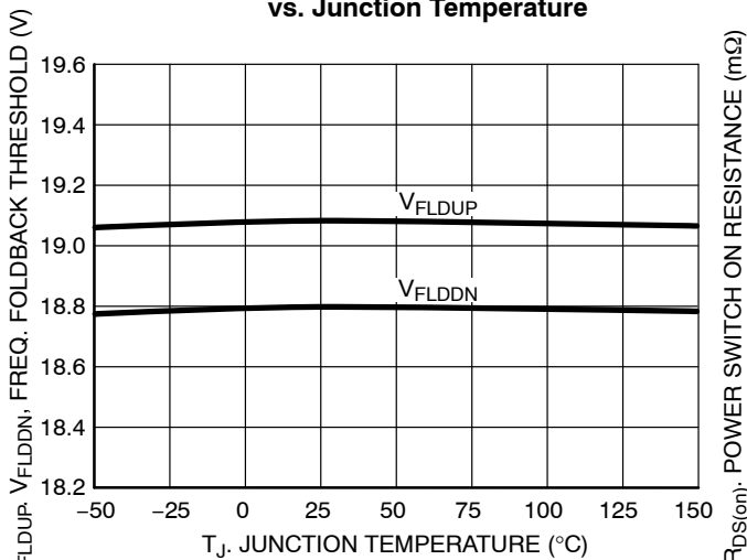
Figure 14. Rising Frequency Foldback Threshold vs. Junction Temperature
