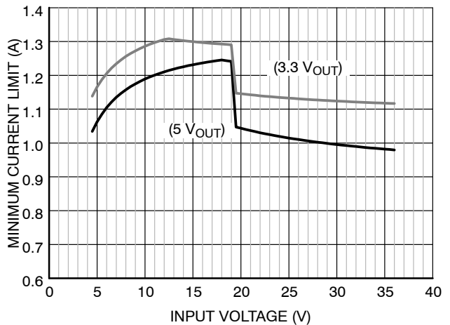
Figure 26. NCV890103 Load Current Capability with 4.7 \mu H Inductor
