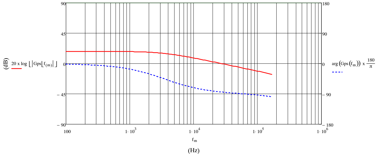
Figure 31. Power Stage Bode Plots
