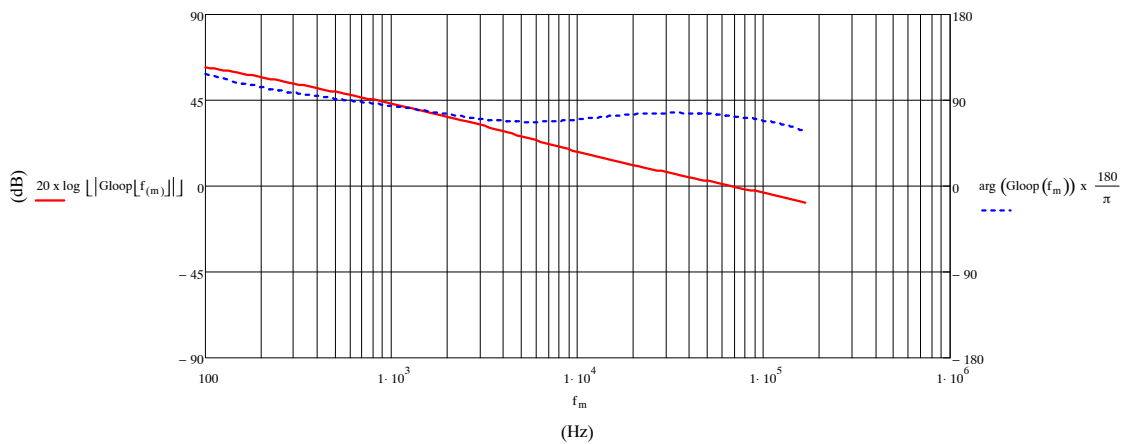
Figure 34. Bode Plot of the Total Loop
