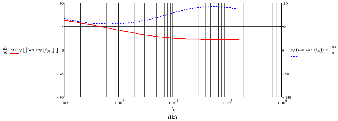
Figure 33. Bode Plot of the OTA Compensator
