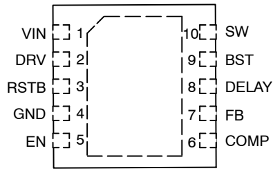
Figure 3. Pin Connections
