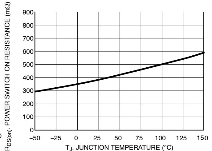
Figure 15. Power Switch R DS(on) vs. Junction Temperature
