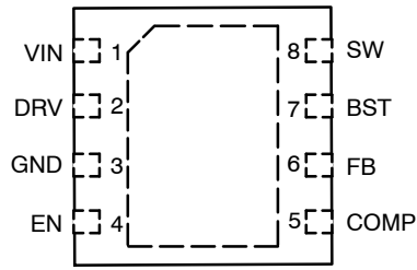
Figure 3. Pin Connections
