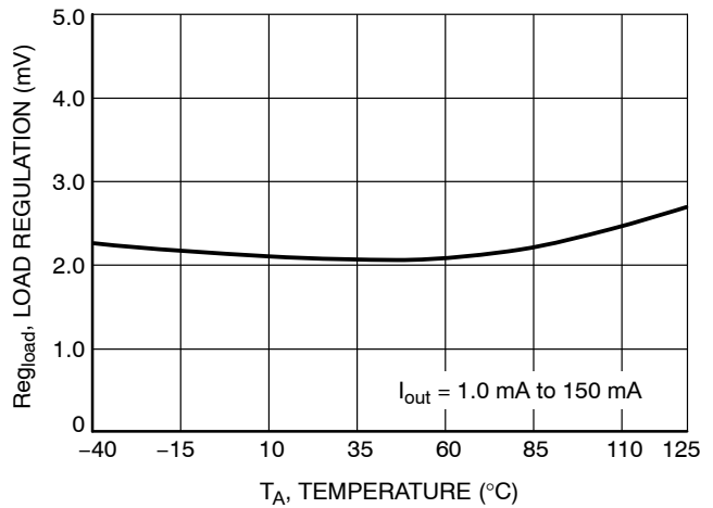
Figure 13. Load Regulation vs. Temperature
