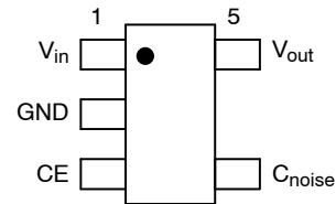
TSOP-5 (Top View)
