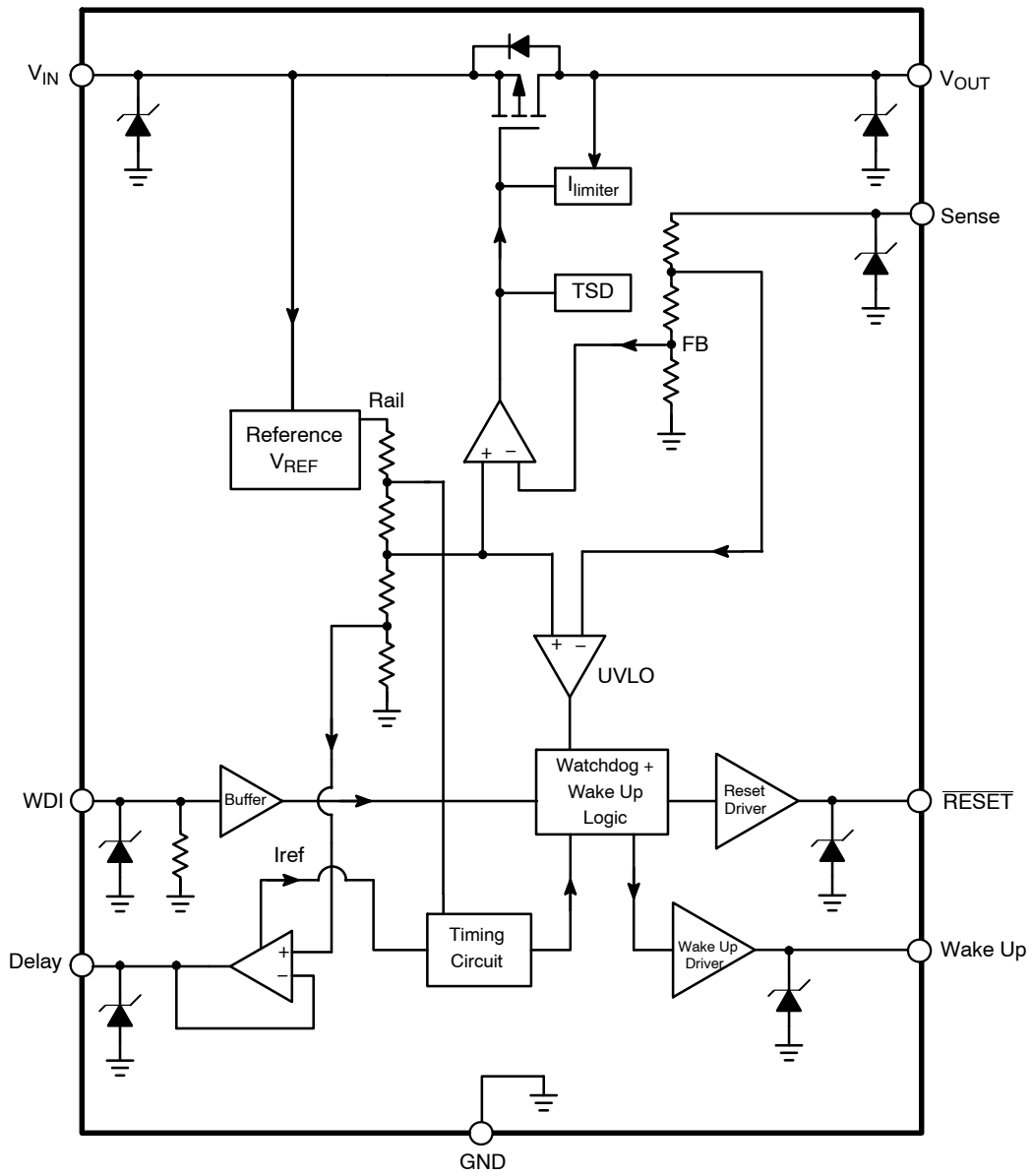
Figure 2. Block Diagram
