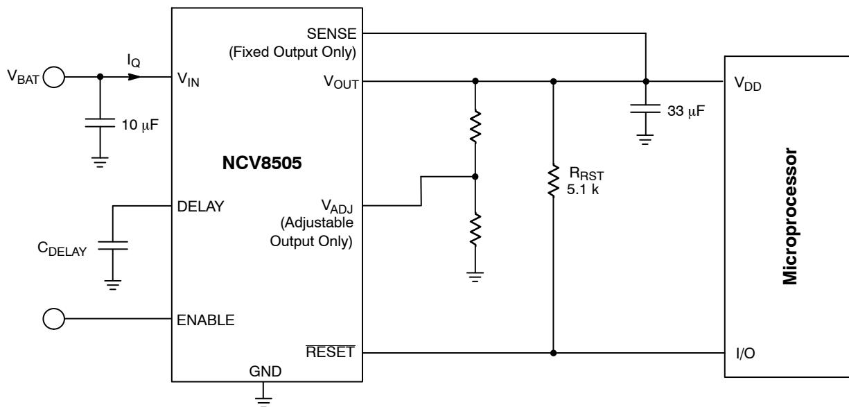
Figure 1. Application Diagram
